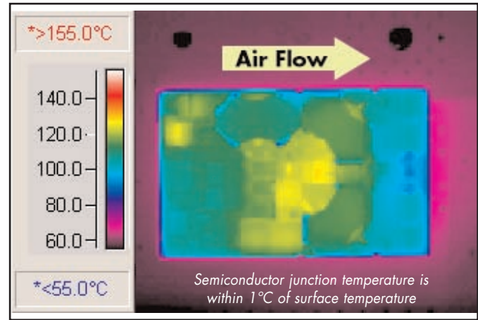
Figure 8: Thermal plot of converter at 6.4 amp load current (77W) with 55^{\circ}C air flowing at the rate of 200 LFM. Air is flowing across the converter from input to output (nominal input voltage).
