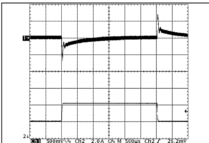
Figure 11: Output voltage response to step-change in load current (50%-75%-50% of I_{out(max)} ; dI/dt = 0.1A/\mu s ). Load cap: 10\mu F , 100 m\Omega ESR tantalum capacitor and 1\mu F ceramic capacitor. Ch 1: V_{out} (500mV/div), Ch 2: I_{out} (2A/div).
