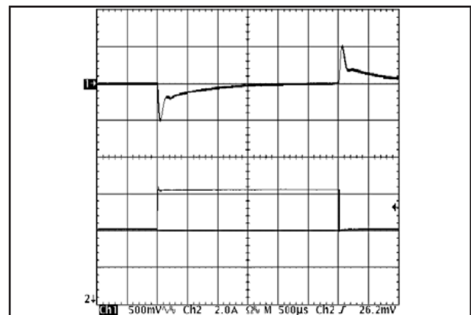
Figure 12: Output voltage response to step-change in load current (50%-75%-50% of I_{out(max)} ; dI/dt = 5A/\mu s ). Load cap: 100\mu F , 30 m\Omega ESR tantalum capacitor and 1\mu F ceramic cap. Ch 1: V_{out} (500mV/div), Ch 2: I_{out} (2A/div).
